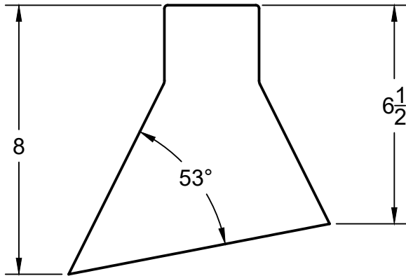
SIDE
